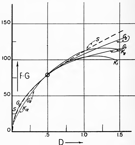
FIG. 14. Comparison of graininess-density functions obtained by different methods and observers. For commensurability all curves have been reduced to an identical G -value for D = 0.5 . The dashed curve ( S ) represents the parabola G \sim d\sqrt{D} ; K_1 , K_2 are by van Kreveld; 9 G_1 , G_2 are identical with those in Fig. 9.
